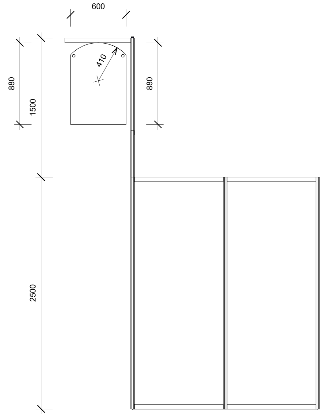
② RIGHT ELEVATION 1:25
