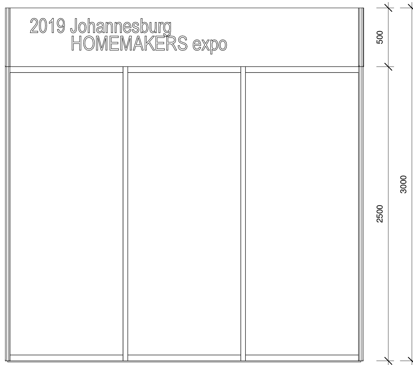
1 FRONT ELEVATION 1:20
