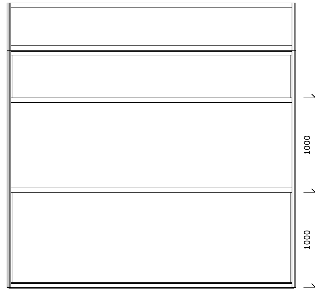
2 BACK ELEVATION 1 : 25
