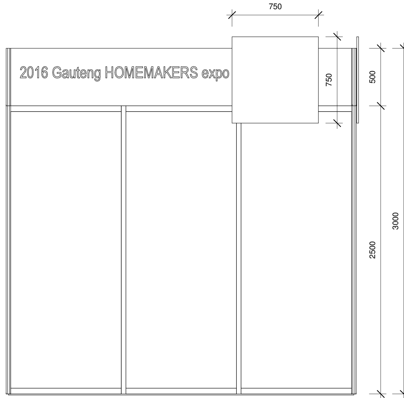
1 FRONT ELEVATION 1 : 20
